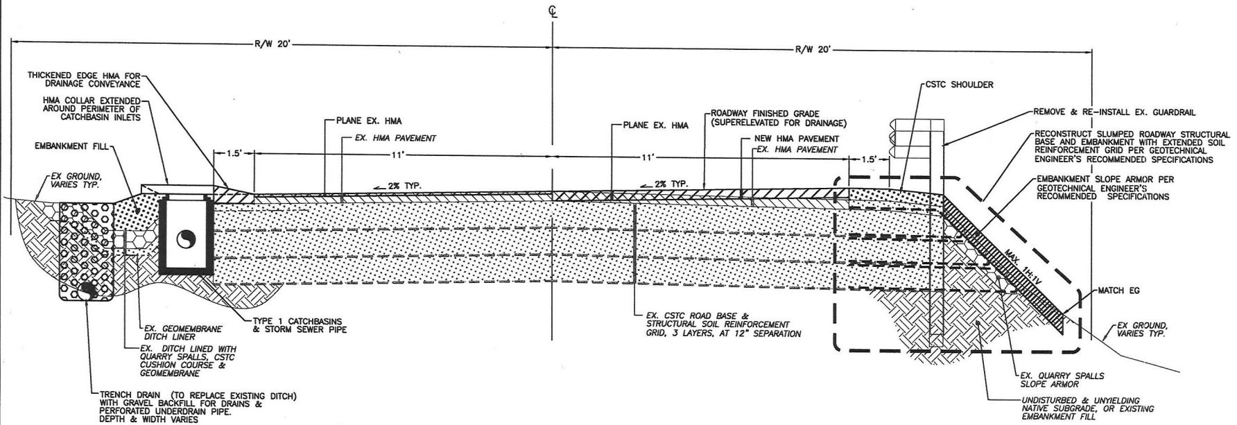
TYPICAL ROADWAY SECTION - SOUTH PASS ROAD REPAIR NOT TO SCALE
