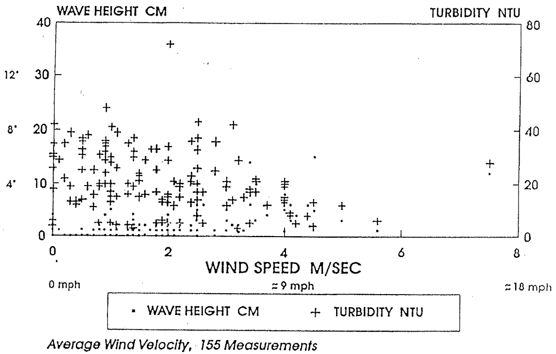
Figure 29. Wave height and turbidity compared to wind speed river channel data 1990-1991
