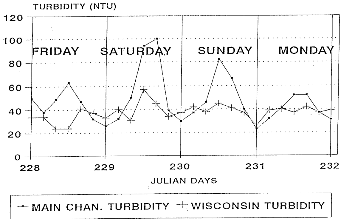
Figure 26. Main Channel and Wisconsin Channel turbidity values August 15-19, 1991
