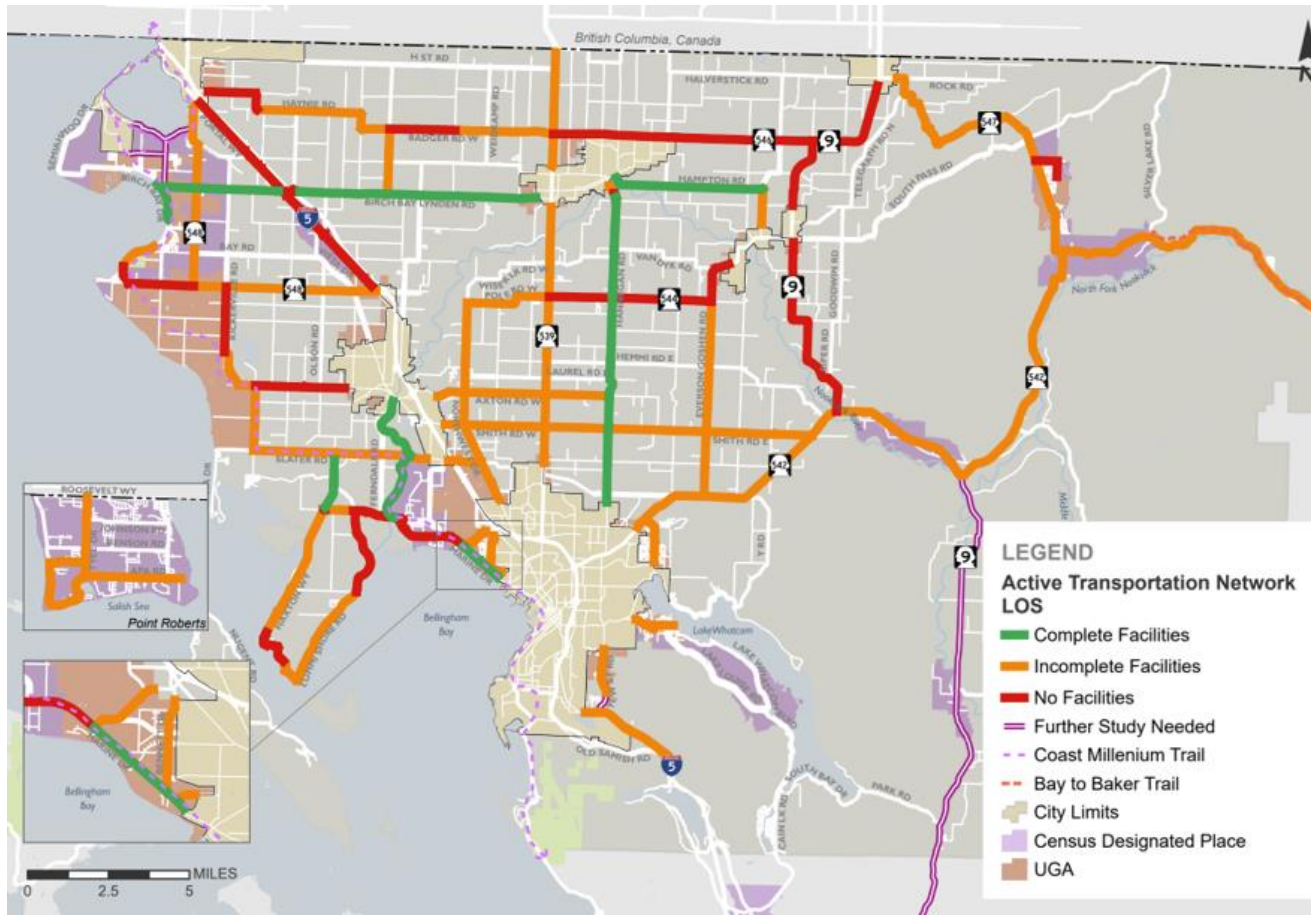
Figure 9.3 Active Transportation Network LOS Status in 2025
